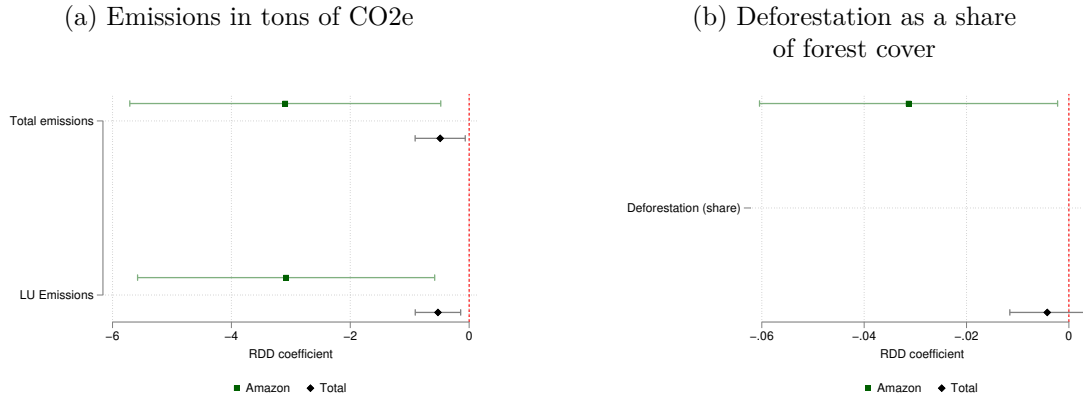
Figure A.9: Excluding Municipalities in the LPM.
