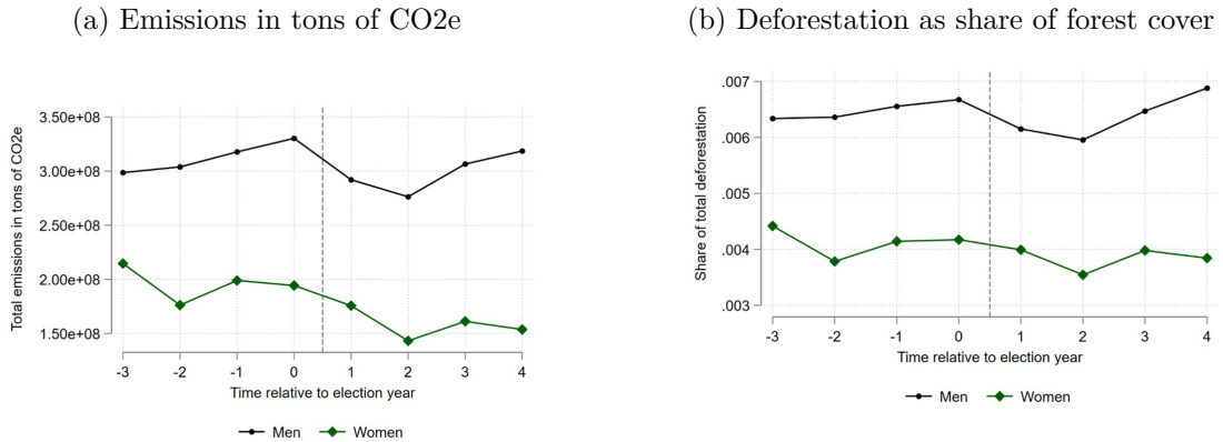
Figure A.5: Evolution of Environmental Outcomes
