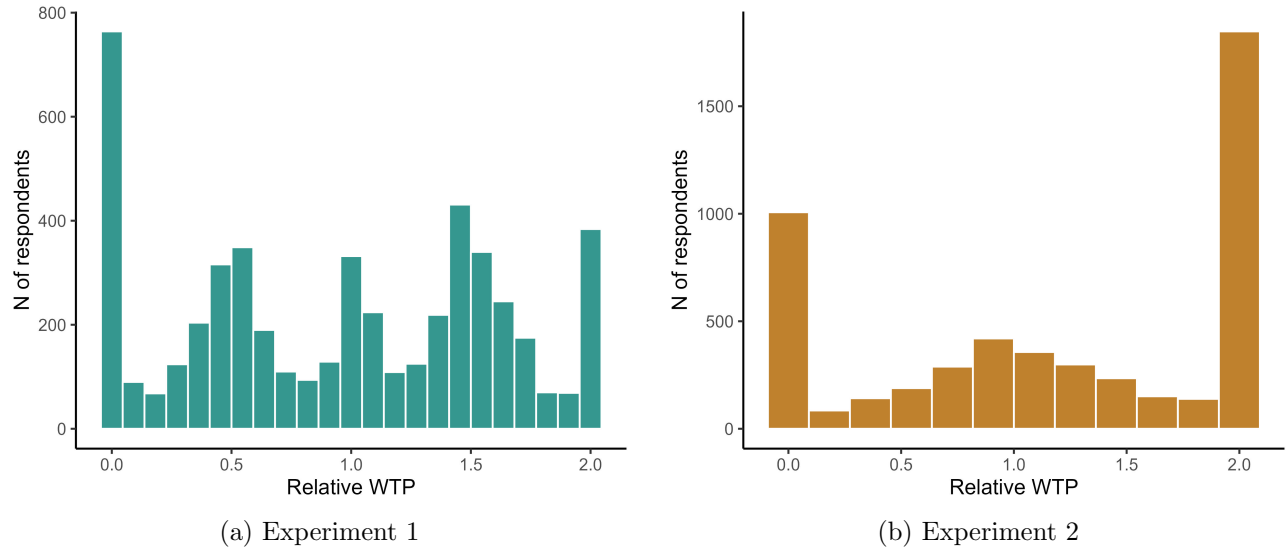
Figure A4. Distribution of relative WTP for safety in public transportation
