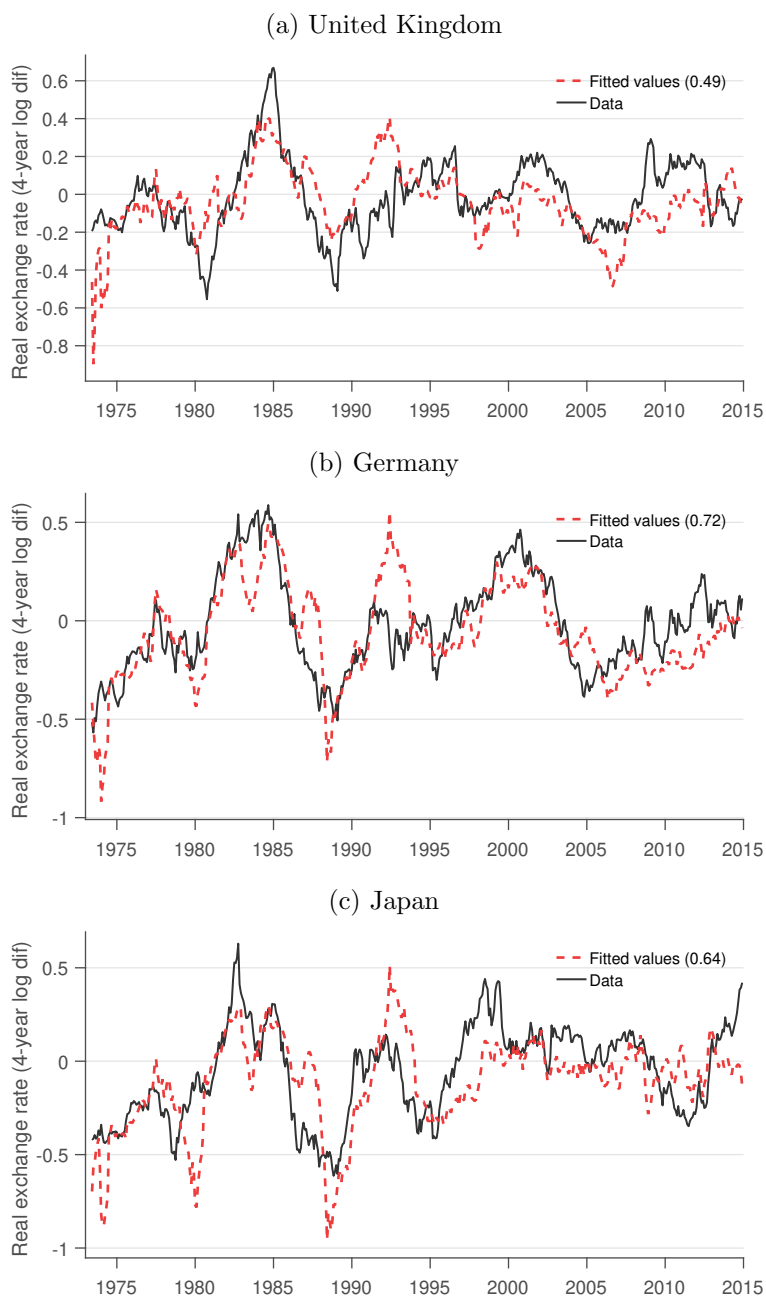
Figure 3: Out-of-Sample Fit Six Months Ahead with Four Commodities (best fit)
