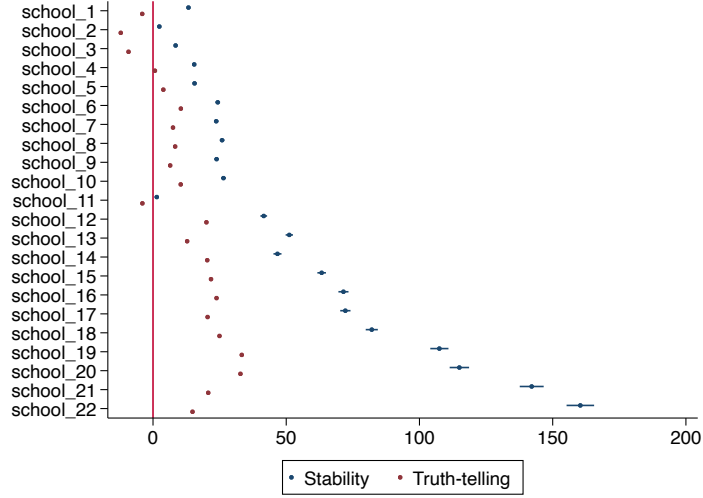
Figure 6: Average tastes in willingness-to-travel ( \frac{\hat{\delta}_j}{\hat{\lambda}} )
