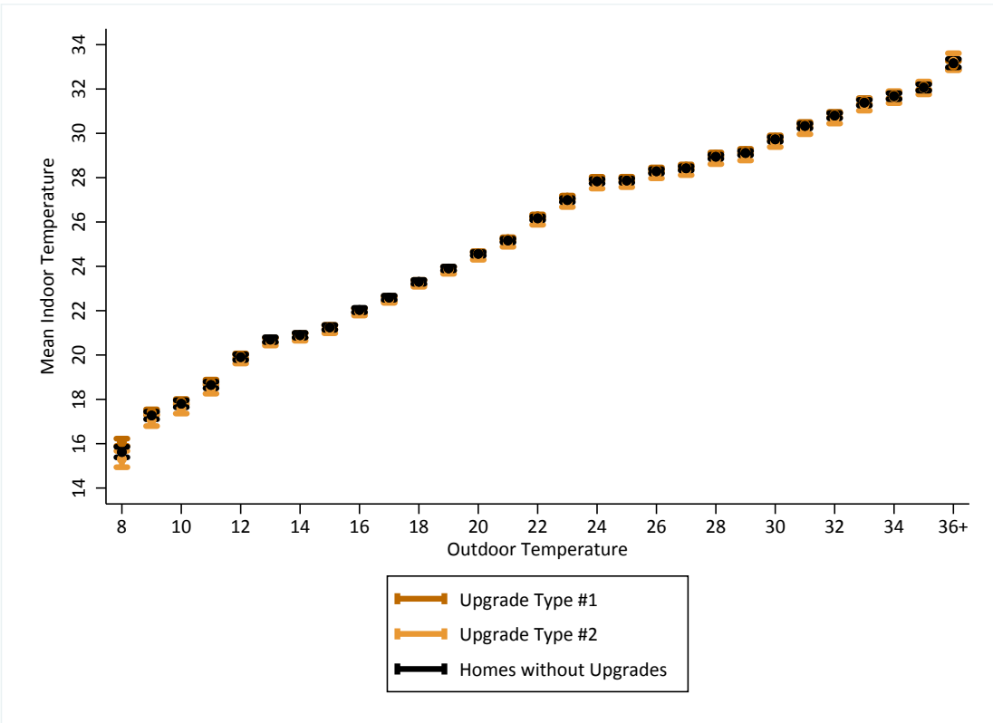
Figure 6: Indoor vs. Outdoor Temperature, By Upgrade Type
