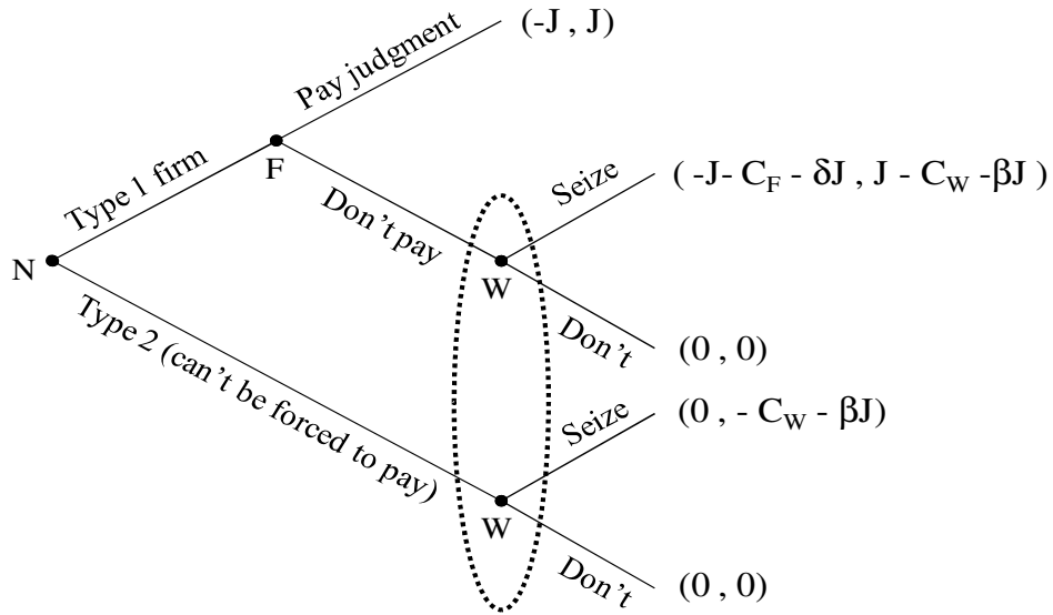
Figure 1. Game Tree
